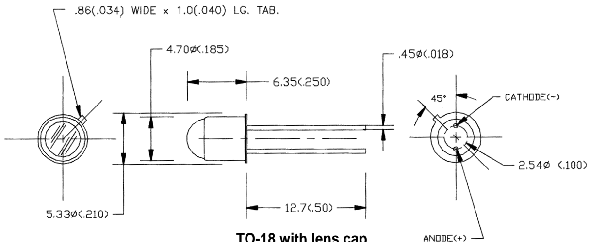
TO-18 with lens cap (Chip Diameter to 2 mm)
